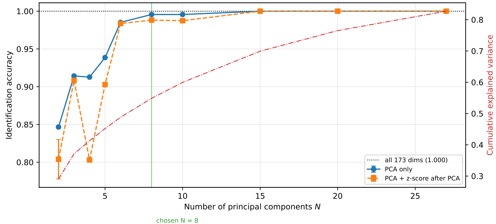
Accuracy and explained variance versus the number of retained components
